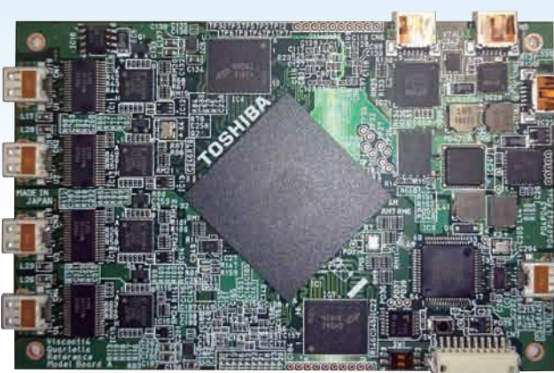
Visconti™ 4 TMPV7608XBG
